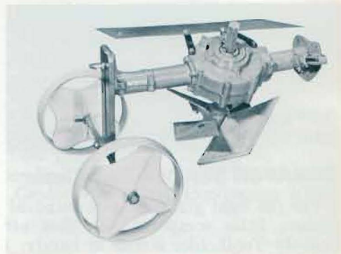
SPECIFICATIONS: 15578E1 Rotary Plow Drive: splined steel shafts, bevel gears, completely enclosed. Plow: four blades, high carbon steel, forged cutting edges.
