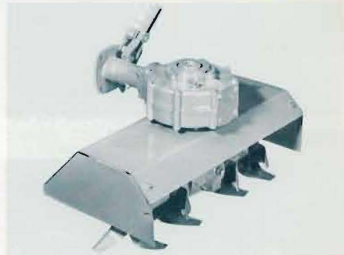
SPECIFICATIONS: 15579E1 Rotary Cultivator Drive: splined steel shafts, gears, fully enclosed. Tines: 16, high carbon steel, forged. Cutting Depth: 3 inches. Width: 26 inches. Height: 19 inches. Length: 10 inches. Attaches to: Rotary Plow Drive Assembly.
